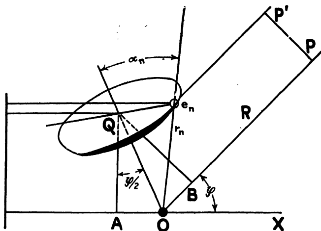
Fig. 7.—Scattering of monochromatic x-rays by an atom of an inert gas.
